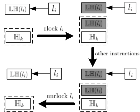
Fig. 4 Ownership Transfer for Acquiring and Releasing Read Lock
